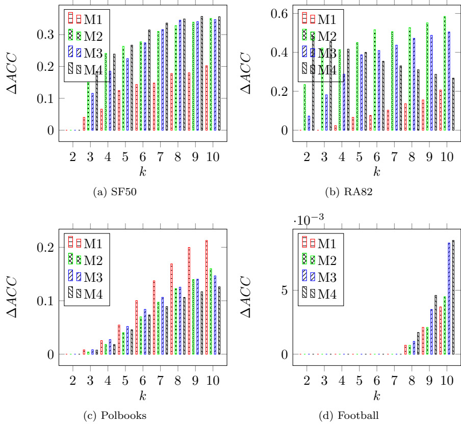
Figure 1: The value of \Delta ACC for different datasets and models in k = 2 \dots 10 .
